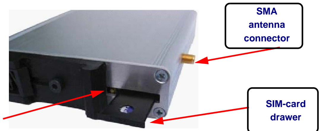
Figure 7: SIM-card insertion
