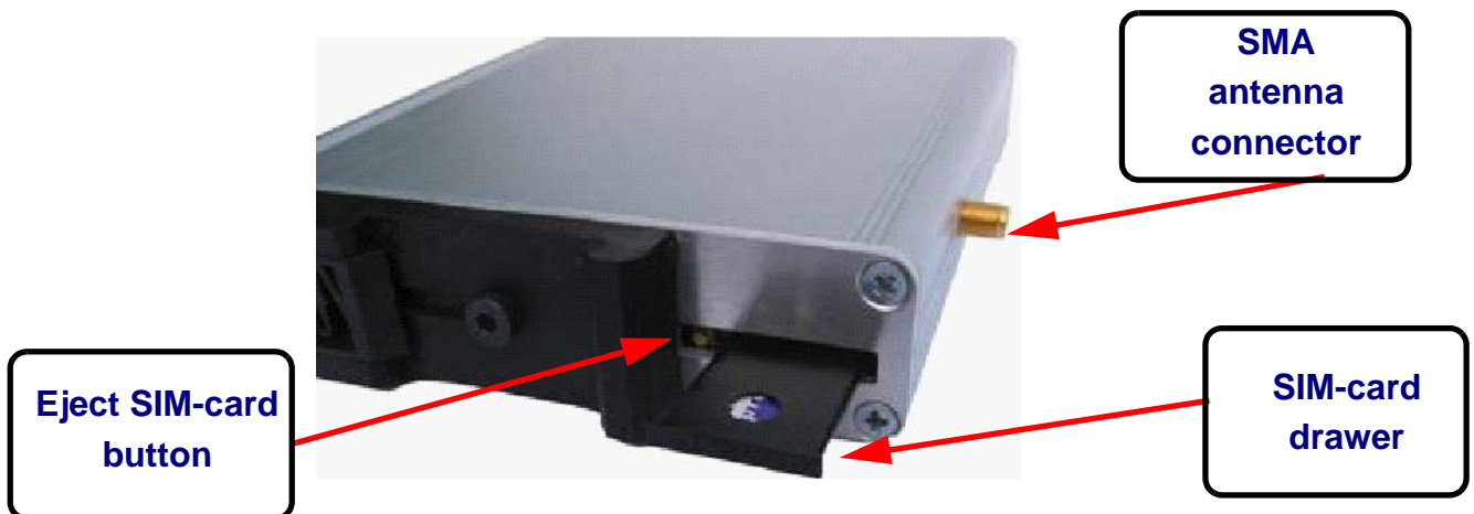
Figure 7: SIM-card insertion
