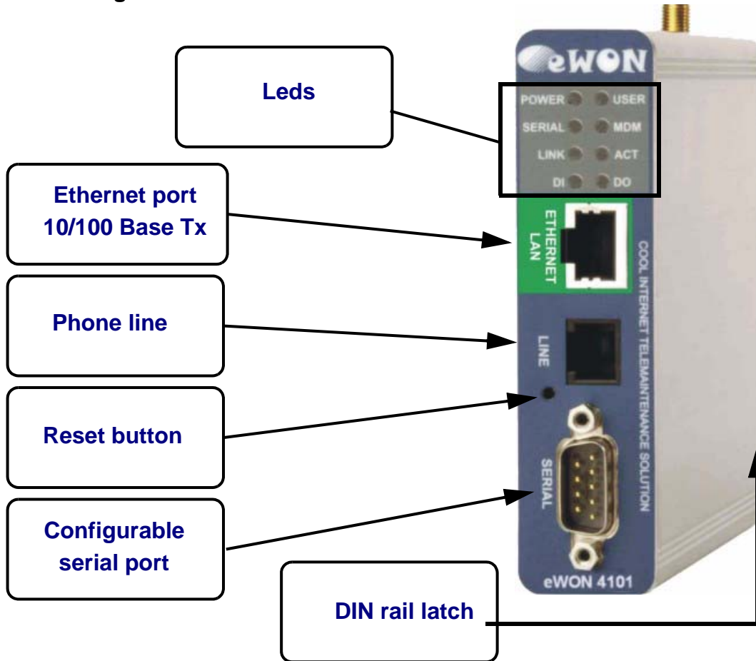
Figure 1: Housing, front view
